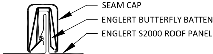
ASSEMBLED BUTTERFLY BATTEN w/ SEAM CAP: SIDE VIEW
