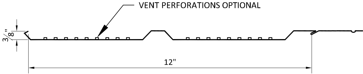
SOFFIT PANEL PROFILE
