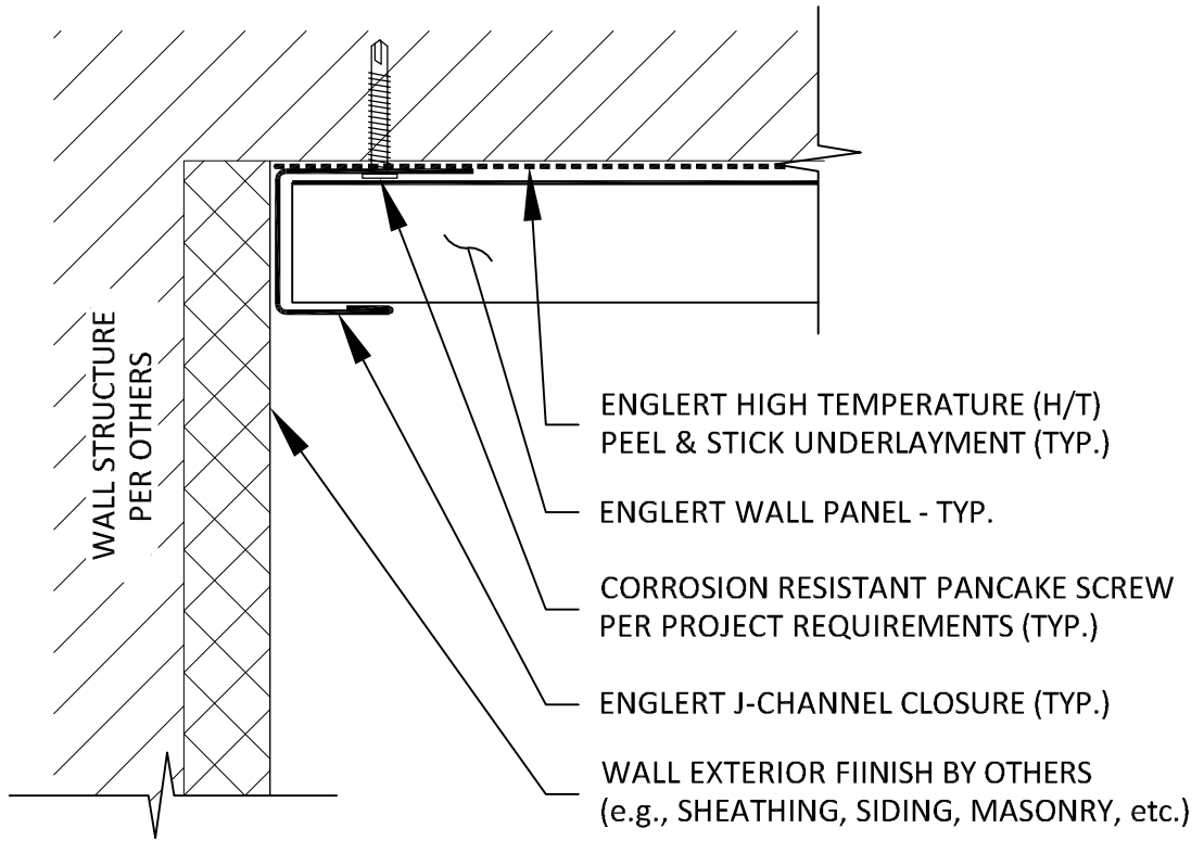
PLAN VIEW
