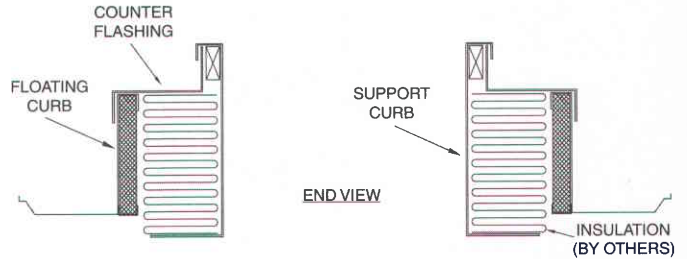
Model #: LMC-TCS (Two-Curb System)
