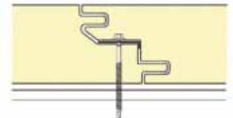
PANEL SIDELAP
