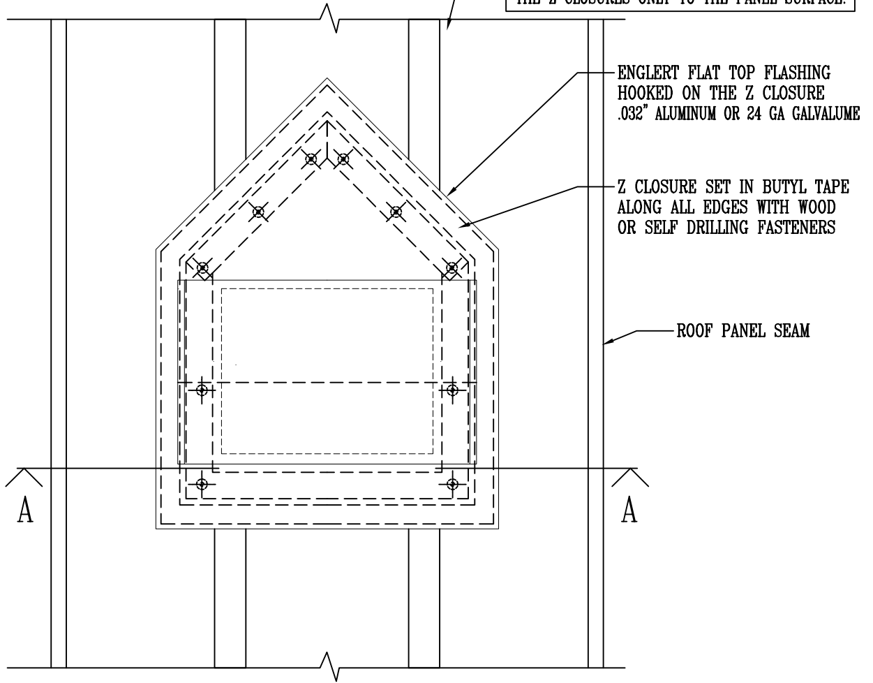
PLAN VIEW
