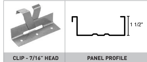
CLIP - 7/16" HEAD
